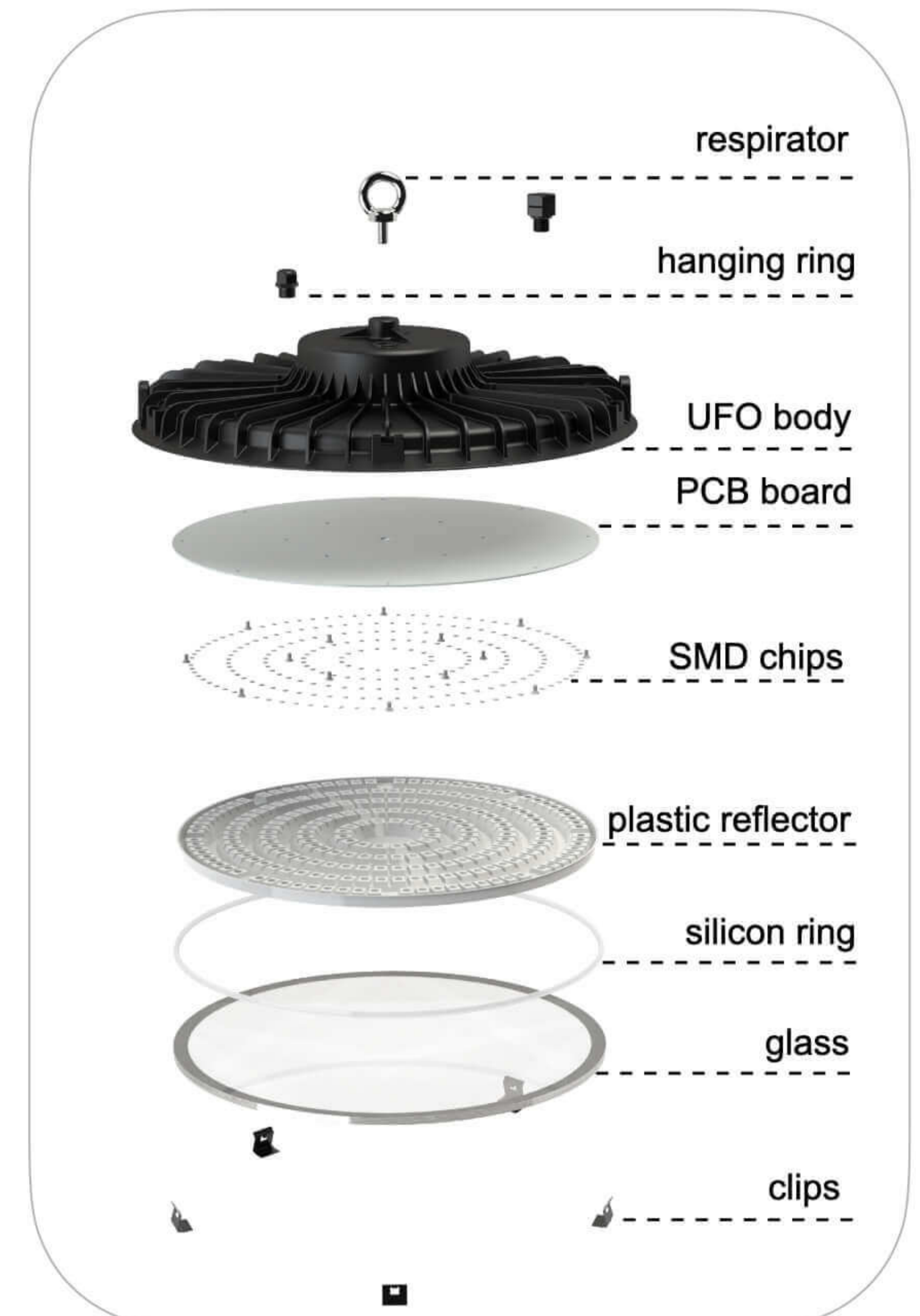
EXPLODED DIAGRAM
